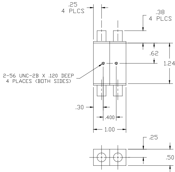
DIMENSIONS (INCHES)
