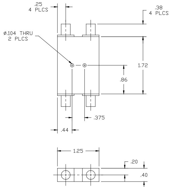
DIMENSIONS (INCHES)
