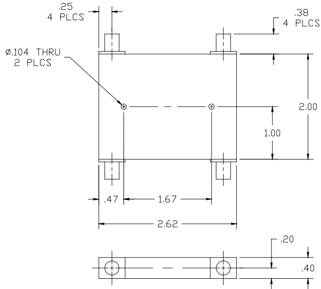
DIMENSIONS (INCHES)
