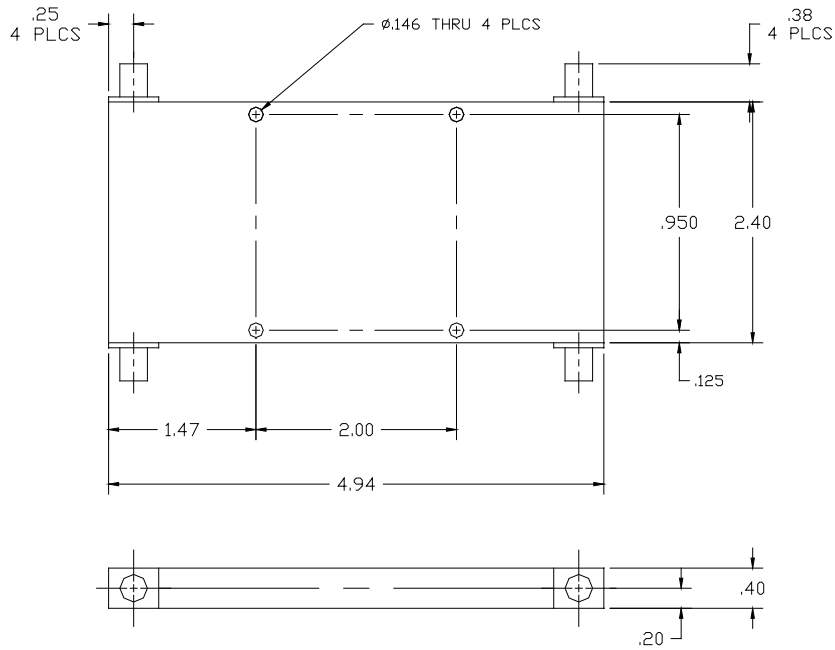
DIMENSIONS (INCHES)
